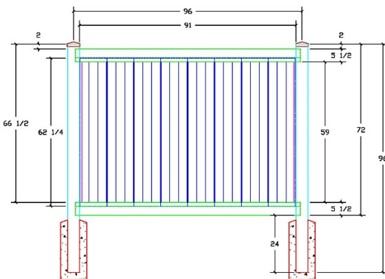
6 FT PRIVACY ON 8 FT CENTERS
