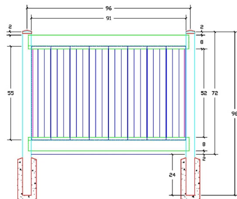
6 FT PRIVACY ON 8 FT CENTERS
